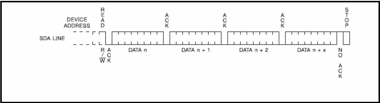
Figure 9. Sequential Read
